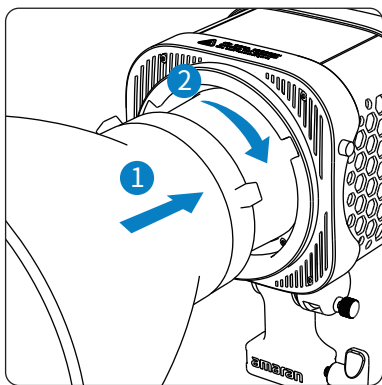
附件安装
